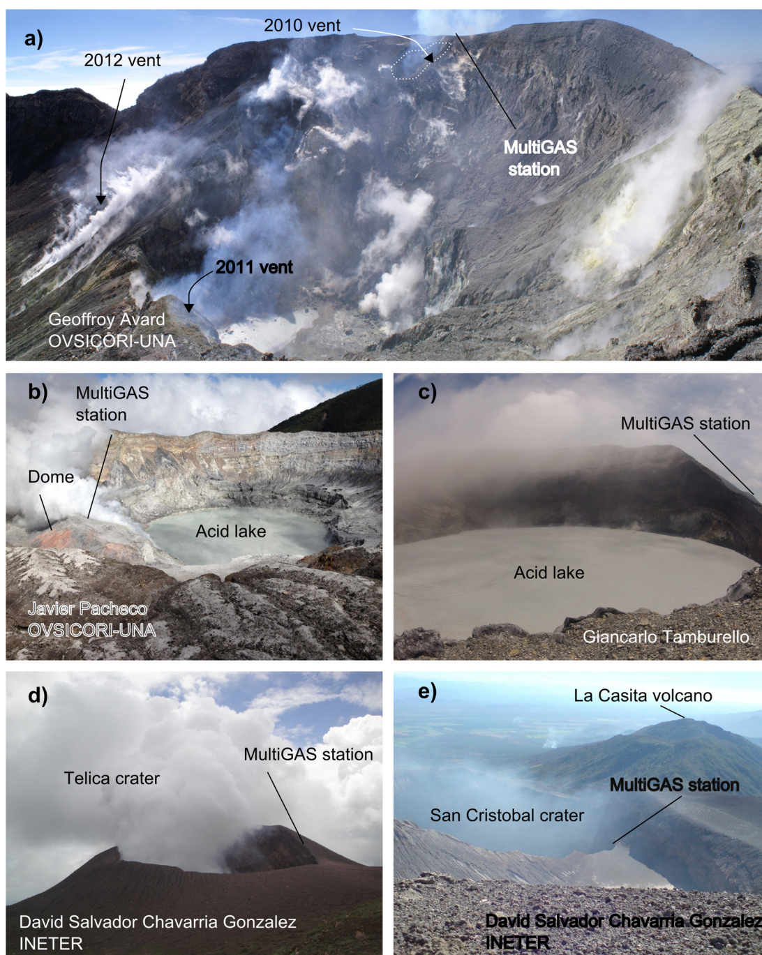
Fig. 2. Degassing activities at the summit craters of the five investigated volcanoes, and the positions of the Multi-GAS instrument: (a) Turrialba, (b) Poás, (c) Rincón de la Vieja, (d) Telica, and (e) San Cristóbal. The credits are shown in the figure.
