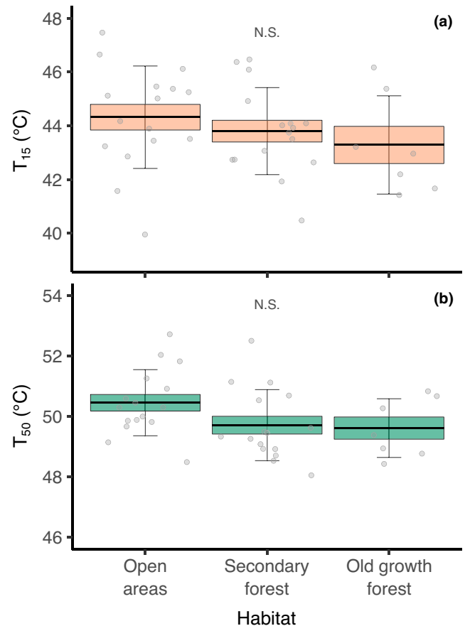
FIGURE 3 Heat tolerance of Zingiberales in open areas, secondary and old growth forest. (a) Critical temperature ( T_{15} ). (b) Temperature at which fluorescence decreases 50% ( T_{50} ). Error bars indicate standard deviation, boxes indicate standard error and the central line represents the average for each habitat. N.S., no significant differences.
