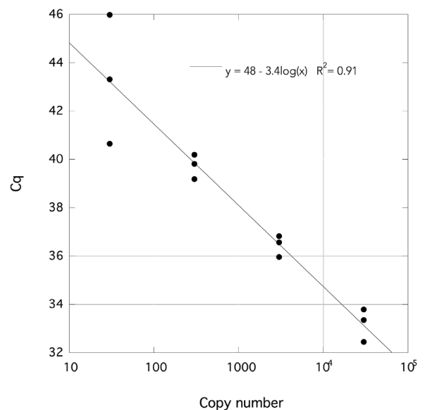
Fig. 5. Standard curve for absolute quantification of T. atroviride BV1CR isolate based on the amplification of DNA serial dilutions (1:10), with the Tatrov oligo set (TrichoBV1 F/TrichoBV1 P/ TrichoBV1 R). The efficiency of the reaction was 98.80 % (Y-intercept = 48.141; Slope = -3.351). The limit of detection (LoD-95 %) was 300 copies of BV1CR DNA.
