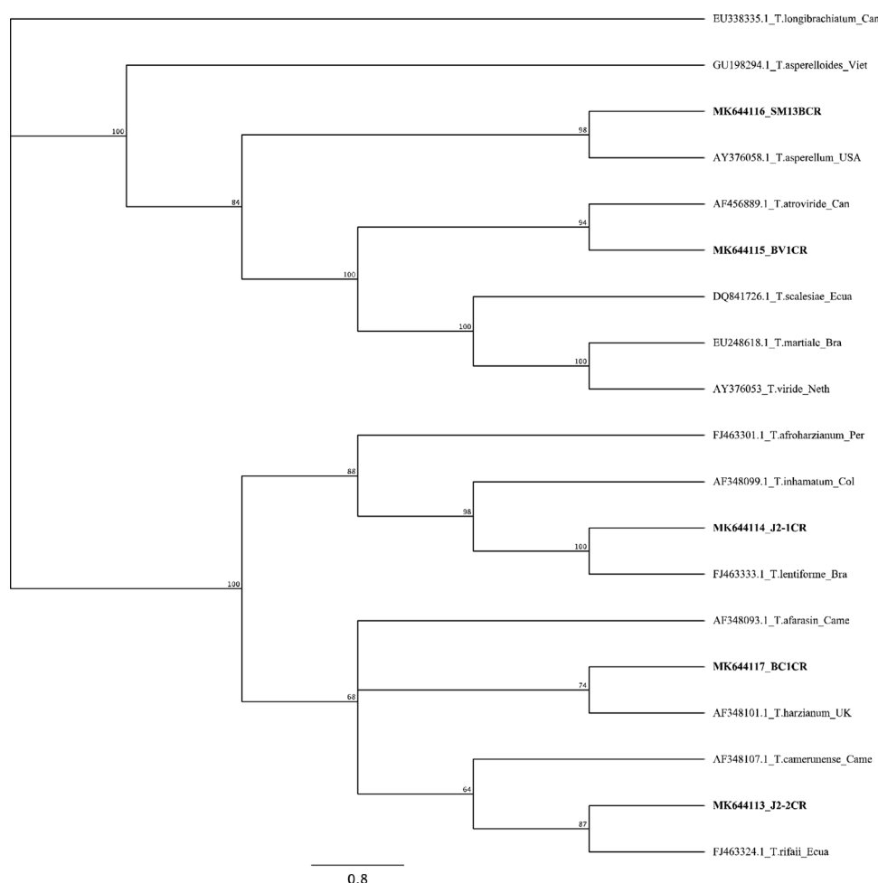
Fig. 2. Phylogenetic tree generated by Mr. Bayes with Bayesian inference based on MAFFT alignment of partial sequences (714 nucleotides) of the tef1-α gene with 1000 replacements, showing the position of different Trichoderma species. Sequences from this study and the GenBank® repository are indicated with the corresponding accession number (countries abbreviated as Bra: Brazil, Can: Canada, Came: Cameroon, Col: Colombia, Ecua: Ecuador, Neth: Netherlands, Per: Peru, UK: United Kingdom, USA: United States, Viet: Vietnam; T. longibrachiatum used as an external group). J2-1CR, BC1CR, J2-2CR, SM13BCR and BV1CR correspond to the isolates identified in this study (CR: Costa Rica).
