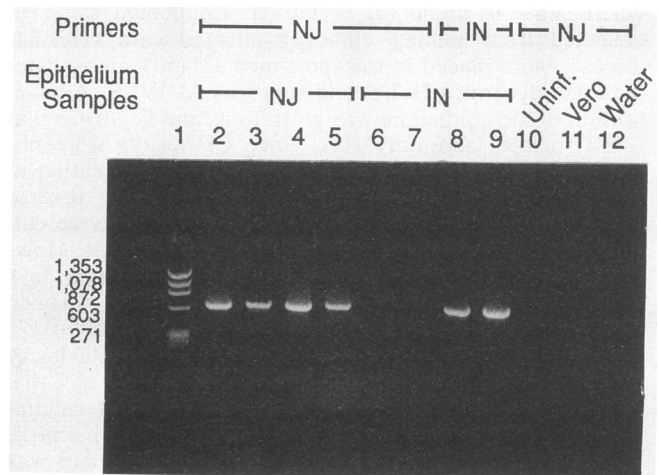
FIG. 2. Agarose gel of products obtained by RT-PCR of epithelium samples from clinical vesicular cases from three provinces of Costa Rica. The samples in lanes 2 to 5 showed typical positive VSV-NJ reactions, showing a 642-bp product band. The samples in lanes 6 to 9 were VSV-IN tested with NJ primers (lanes 6 and 7) or IN primers (lanes 8 and 9). The sample in lane 10 was epithelium from an uninfected (uninf.) cow, and lanes 11 and 12 contain uninfected Vero cells and water (control), respectively. Markers in lane 1 were \phi\text{X174} replicative-form DNA digested with Hae III. The numbers to the left of the gel are the sizes (in base pairs) of size markers.
