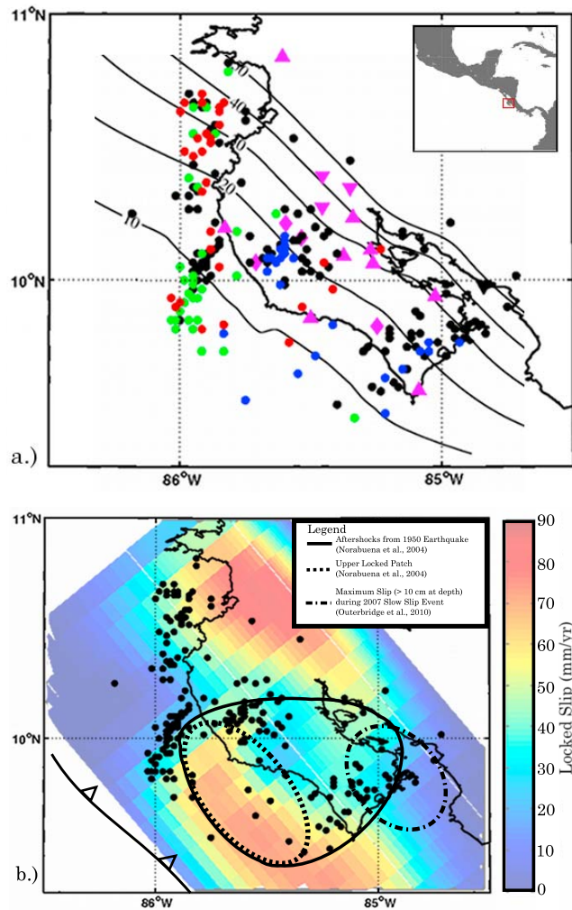
Figure 1. (a) Map of tremor locations color coded to correspond to the temporal record of tremor activity from Figure 3a, including major (blue-May 2007, green-August 2008, and red-April 2009) and minor (black) tremor events. Seismic stations are indicated by the magenta symbols with inverted triangles and diamonds representing borehole and deep vault sites, respectively. The black inverted triangle indicates the location of Puntarenas. (b) Contours of locked slip on the plate interface from Outerbridge [2010] with all tremor locations in black. The plate rate approaches \sim 90 mm/yr [Norabuena et al., 2004]. The aftershock area of the 1950 Nicoya Peninsula Earthquake (Ms 7.7), the shallow locked patch determined by episodic GPS measurements [Norabuena et al., 2004], and the region of maximum slip at depth (greater than 10 cm) during the 2007 Slow Slip Event [Outerbridge et al., 2010] are also indicated.
