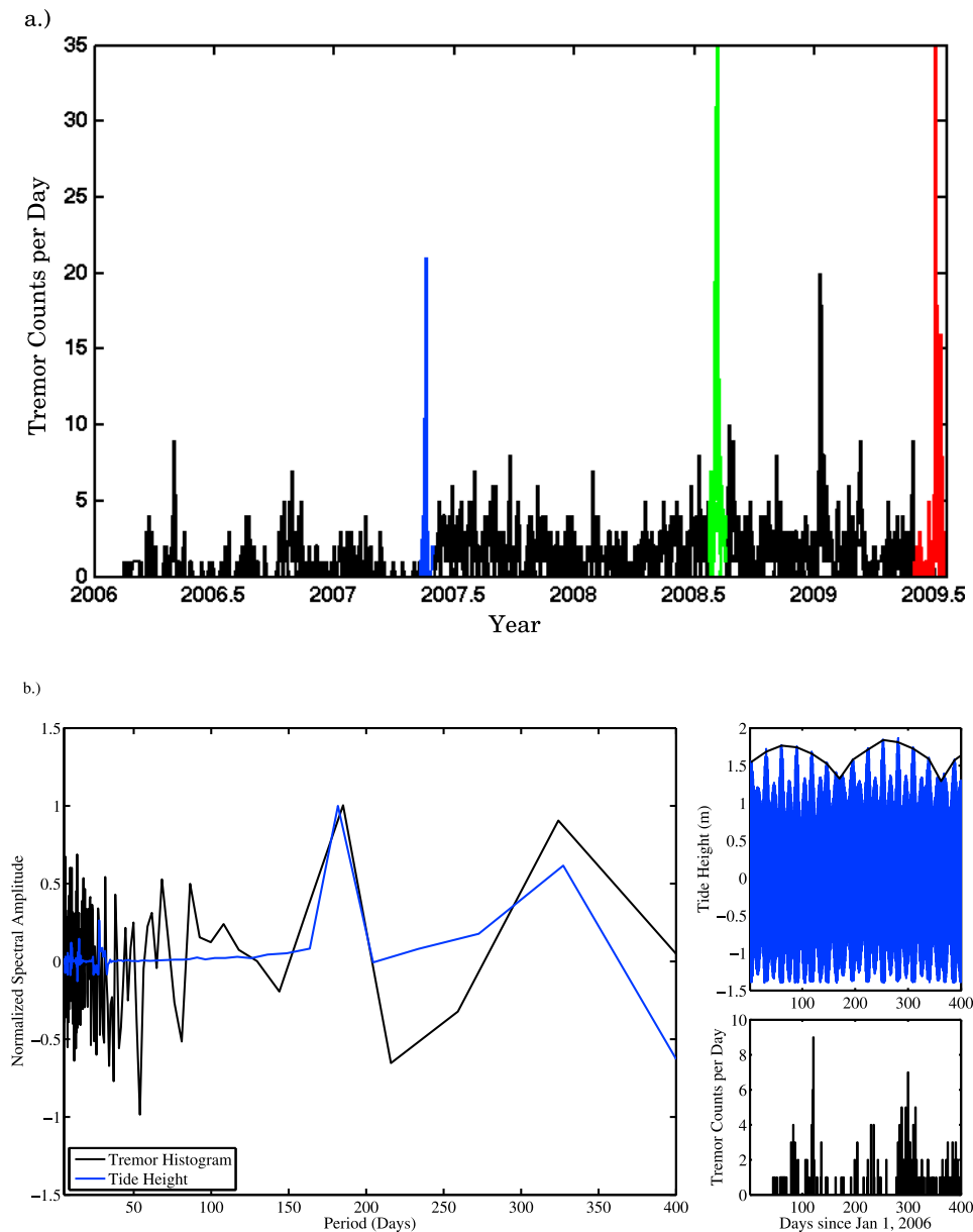
Figure 3. (a) Tremor histogram of daily events from 2006 through mid-2009. Three of the major tremor episodes are color-coded and event locations indicated in Figure 1 (blue for May 2007, green for August 2008, and red for April 2009). (b) (left) Spectra computed for the 2006–2009 tremor and tide height records calculated for Puntarenas, Costa Rica. (right) The 2006 tremor and tide height data to highlight the 180 day periodicity.
