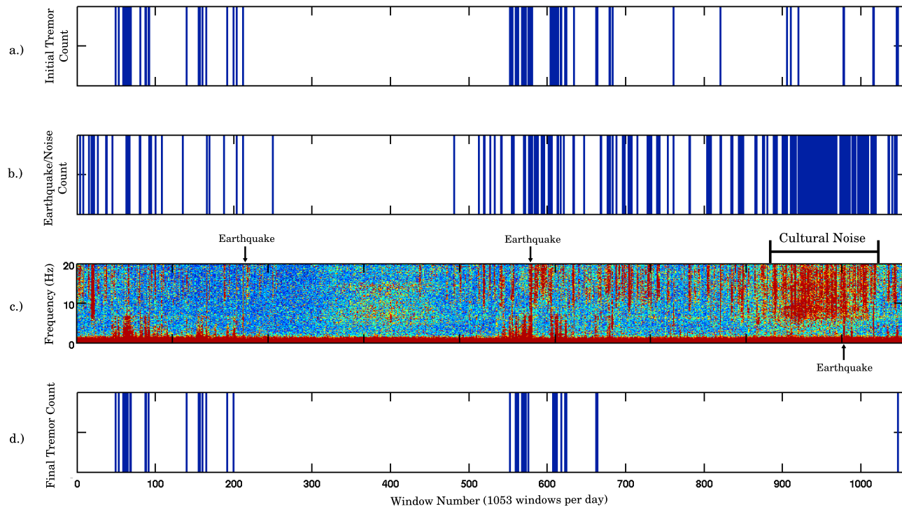
Figure 2. Illustration of the spectral detection method for one day (2008 JD 215) showing (a) initial tremor detections, (b) earthquake and cultural noise detections, (c) the daily stacked network-wide spectrogram with the color axis saturated at the detection threshold (red), and (d) final tremor detections determined by subtracting Figure 2b from Figure 2a. The high level of cultural noise and several earthquakes are indicated on the spectrogram.
