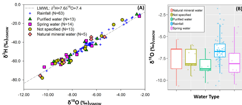
Fig. 1. (A) Dual water isotope diagram including bottled waters classified as purified water (triangles), spring water (squares), natural mineral water (rhombi), and samples in which the water type appeared as not specified (circles). The LMWL of Costa Rica [8] was included as reference. Blue crosses denote the precipitation-weighted mean annual composition across 63 monitoring stations in Costa Rica [7,8]. (B) \delta^{18}\text{O} (in ‰) scattered/box plots per water type, including rainfall values of 63 monitoring stations in Costa Rica [7,8] as a reference. \delta^{18}\text{O} (in ‰) scattered/box plots include 25th, 75th, median, and outliers for each water type.
