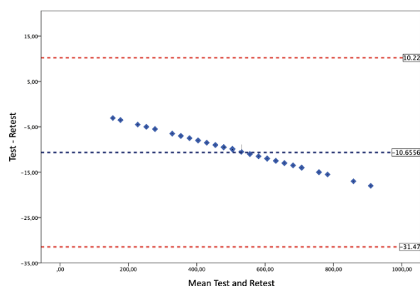
Figure 3. Bland Altman plotting of Test vs Retest.
