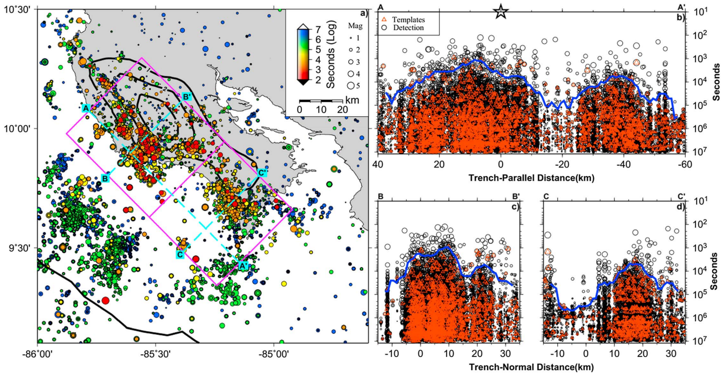
Figure 6. Migration of the 2012 Nicoya aftershocks. (a) Map view of all the detected events color coded by the logarithmic time after the main shock (white star). The thick black contour denotes the 1 m coseismic slip [Kyriakopoulos and Newman, 2016]. (b) The occurrence times of aftershocks since 2012 Nicoya main shock (open black thick star) versus trench-parallel distances (AA'). The black circles and red triangles mark the events listed in the template catalog and detected by the match filter technique, respectively. Blue thick line indicates the activation of aftershock, following Kato and Obara [2014]. (c) The occurrence times of aftershocks within the earthquake group to the northwest since the main shock versus trench-normal distances (BB'). (d) The same as Figure 6c for the earthquake group to the southeast (CC').
