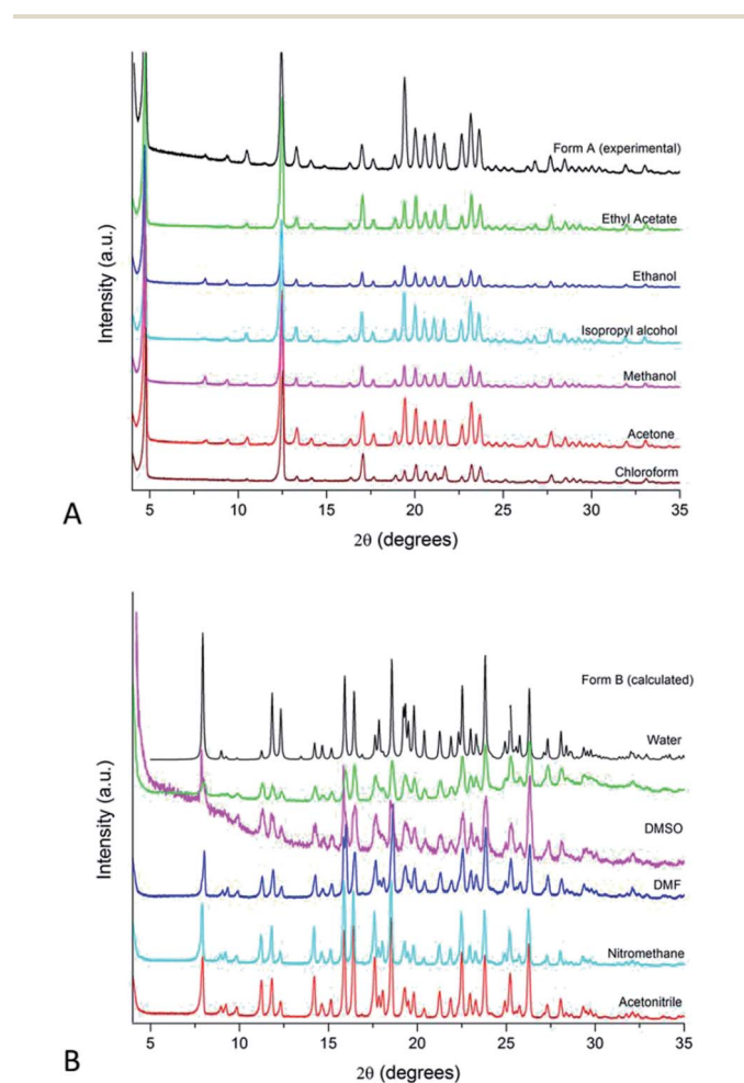
Fig. 1 PXRD patterns of IBS samples grown from solution evaporation at 25 °C: (A) Form A and (B) Form B. The calculated pattern of Form B and the experimental pattern of Form A (commercial raw material) is added for comparison.
